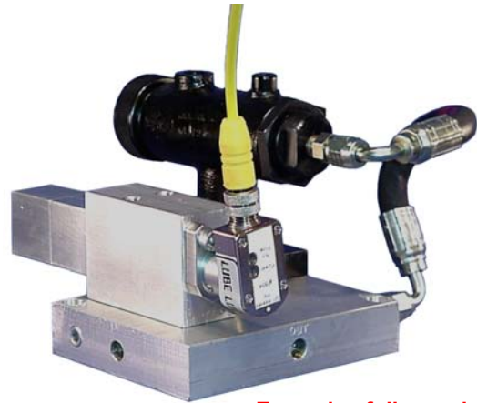
Example of dispensing unit and flow sensor
